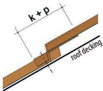
Panels horizontal overlap
